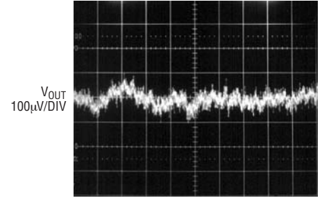
C_{OUT} = 10\mu F 1ms/DIV 3024 G44 I_L = 100mA V_{OUT} SET FOR 5V
