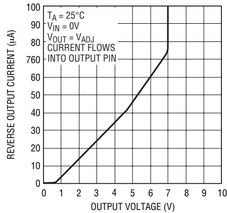
Figure 7. Reverse Output Current
